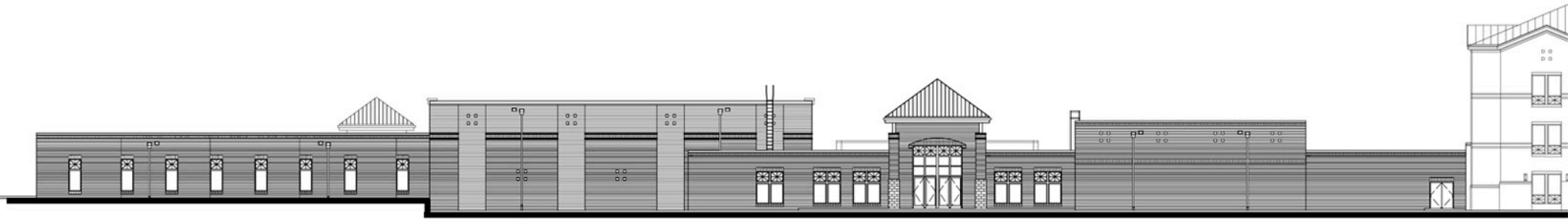
front elevation
